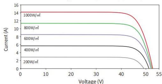
Current-Voltage Curves (72HL4-(V) 595W)
