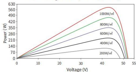
Power-Voltage Curves (72HL4-(V) 595W)
