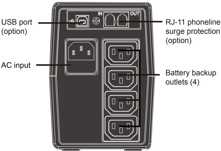
Figure 2 – Rear Panel
